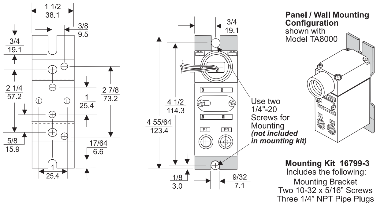
Figure 2. Mounting Kit 16799-3 (Included with unit)
